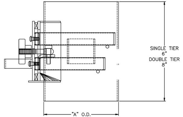
RSDM MOUNTING OPTIONS (BOTH ENDS)
