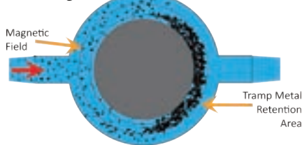
3" Tube Design
