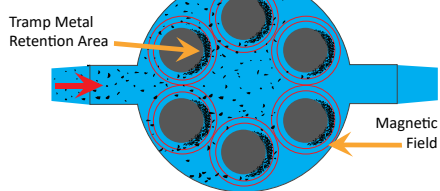
3" Tube Design
